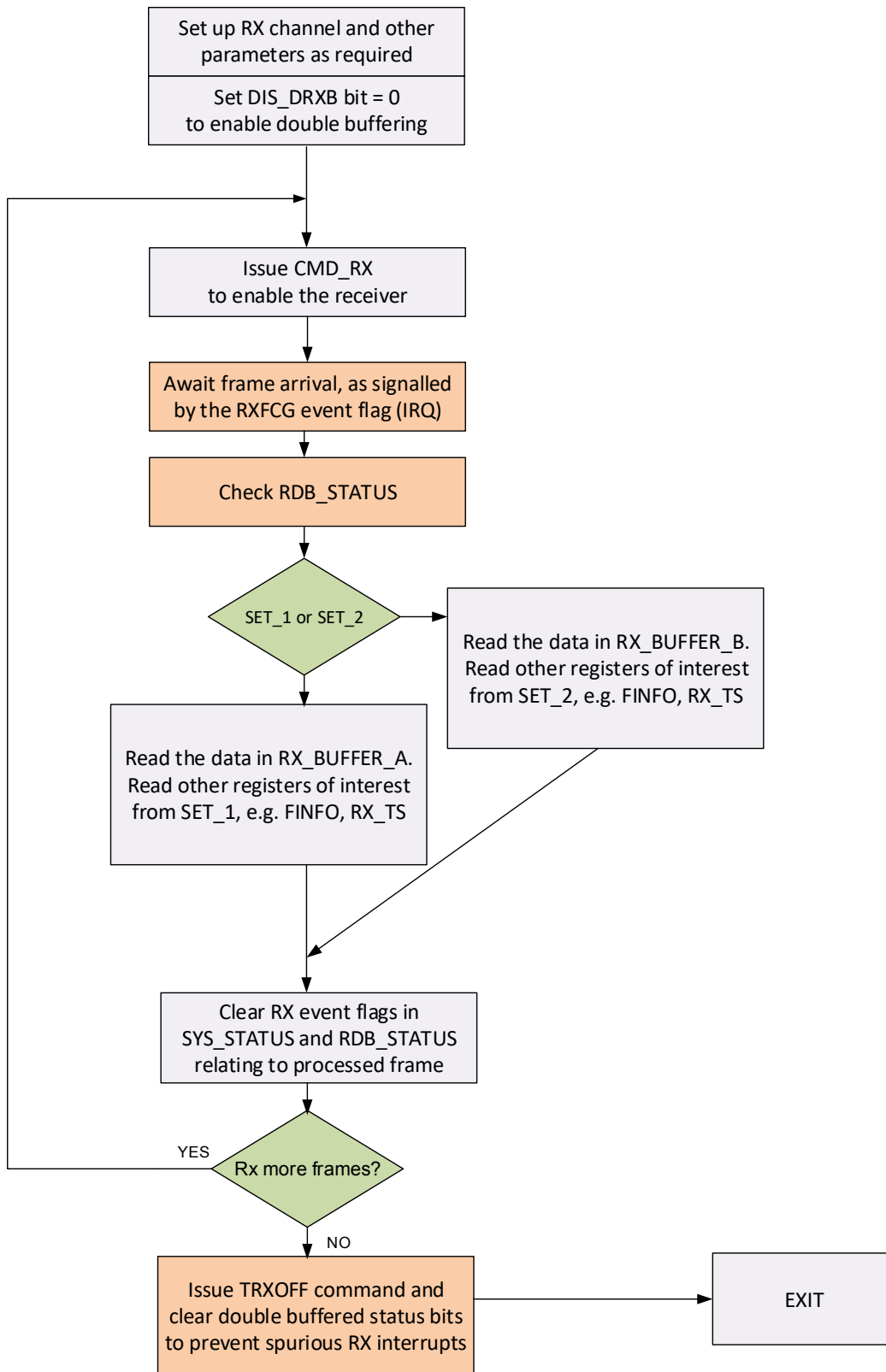
Figure 17: Flow chart for using double RX buffering
